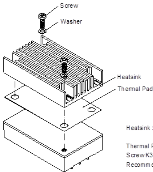
Figure 4 Installation Drawing
