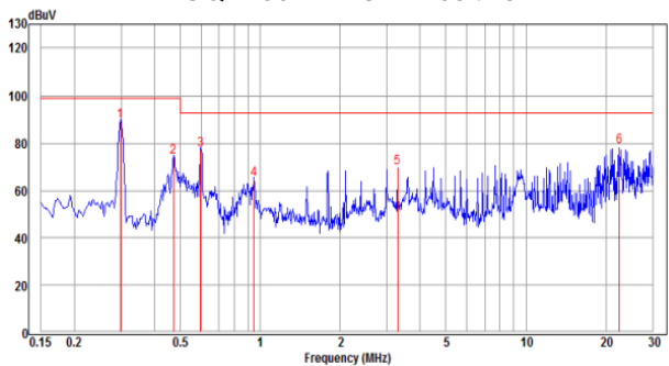
CQB150W-48S24 Positive
