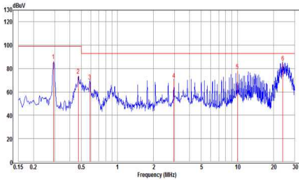
CQB150W-24S24 Positive
