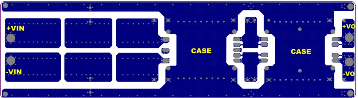
EMI test board bottom side
