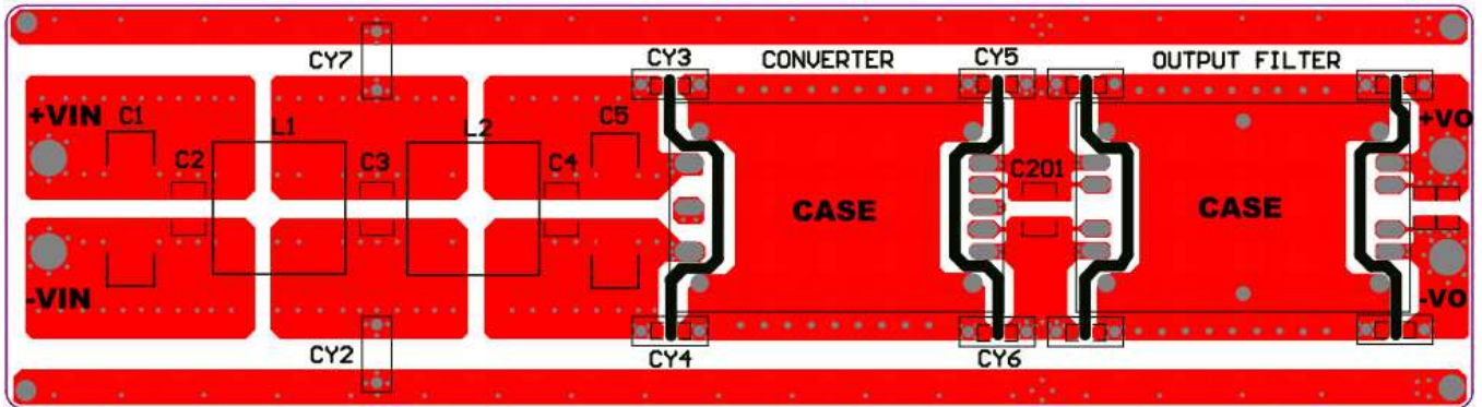
CONVERTER
