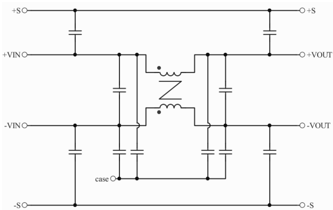
Figure1 Internal Schematic for FM30R080P Module
