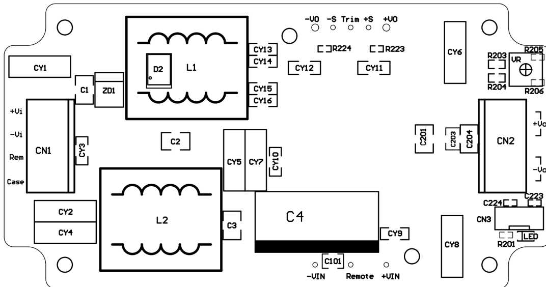
Figure2 Component Placement
