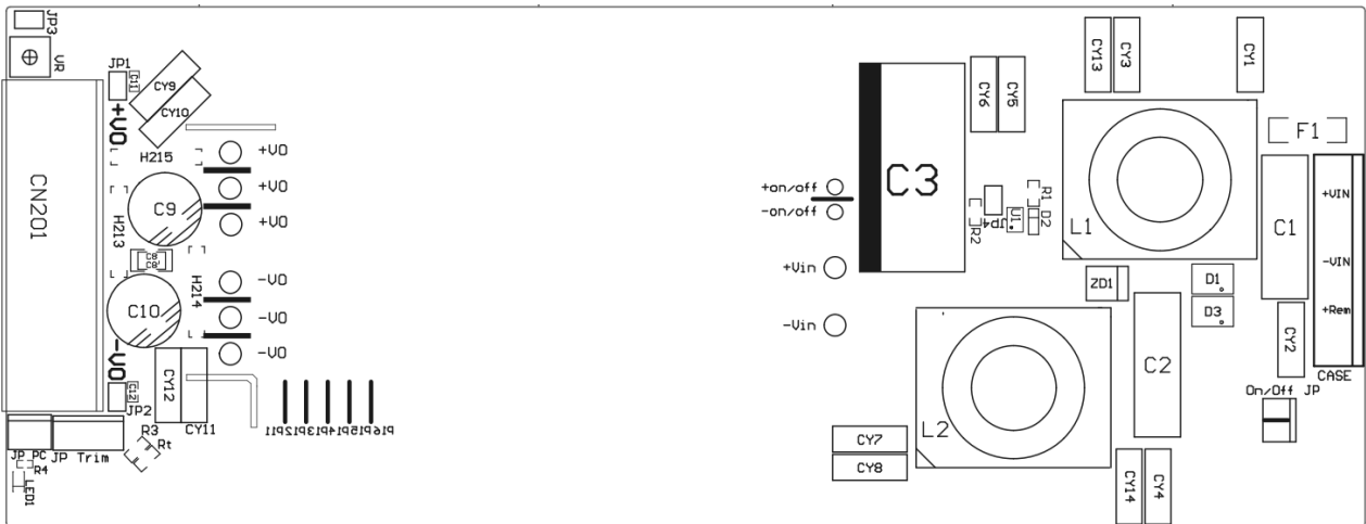
Figure2 Component Placement
