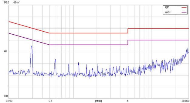
Conducted Class B of EC3SAW-24S33HP
