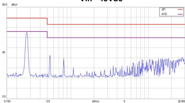
Conducted Class A of EC3SAW-48D15HP
