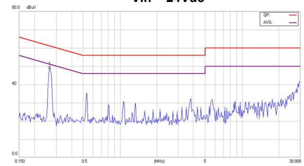
Conducted Class B of EC3SAW-24S05HP
