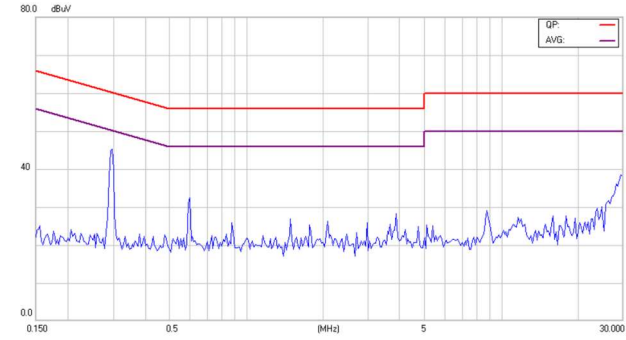
Conducted Class B of EC3SAW-24S12HP
