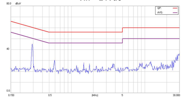
Conducted Class B of EC3SAW-24S15HP
