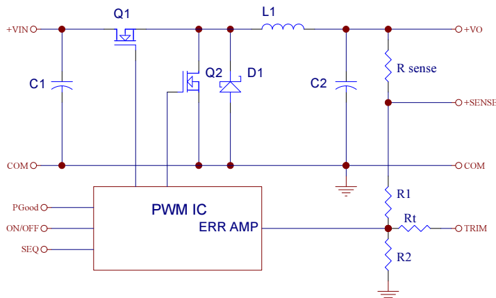
Figure 1. Simplified Schematic
