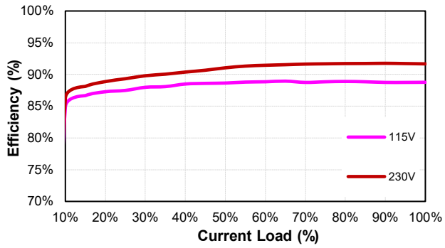
PDF700S560-CMFC/D/D-P (Eff Vs Io)
