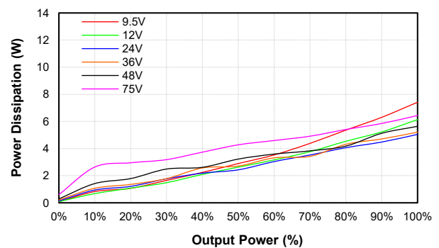
CQB50W8-36S12-CMFC Pd Vs Po @25 Deg. C
