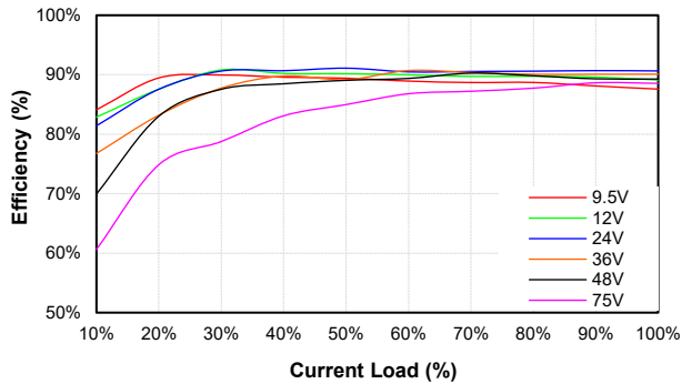
CQB50W8-36S24-CMFC Eff Vs Io @25 Deg. C
