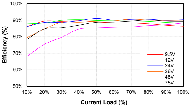
CQB50W8-36S15-CMFC Eff Vs Io @25 Deg. C
