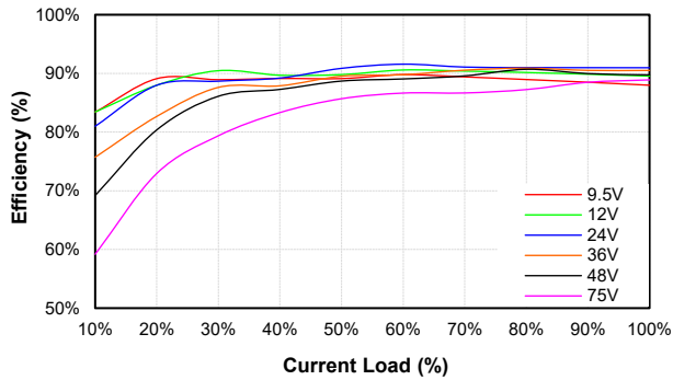
CQB50W8-36S28-CMFC Eff Vs Io @25 Deg. C
