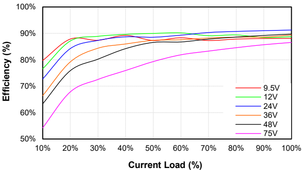
CQB50W8-36S48-CMFC Eff Vs Io @25 Deg. C
