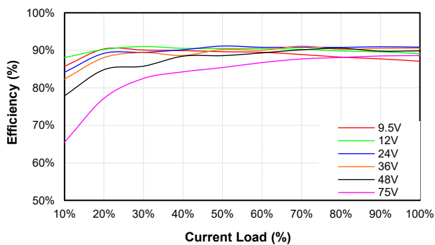
CQB50W8-36S12-CMFC Eff Vs Io @25 Deg. C
