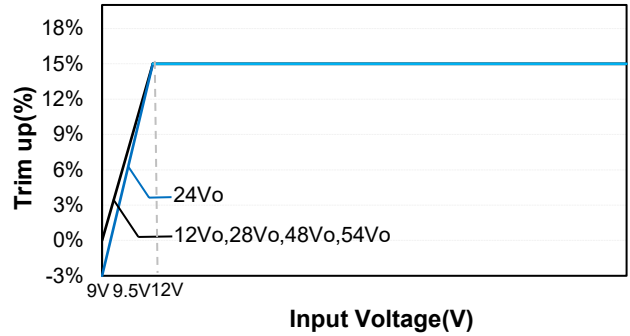
Trim up VS Input Voltage
