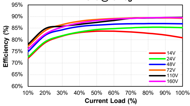
CHB200W12-72S48 Eff Vs Io @25 Deg. C
