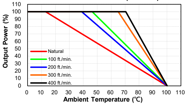
CHB150W12-72S Derating Curve with Heatsink HBT127 (Vin=72V)
