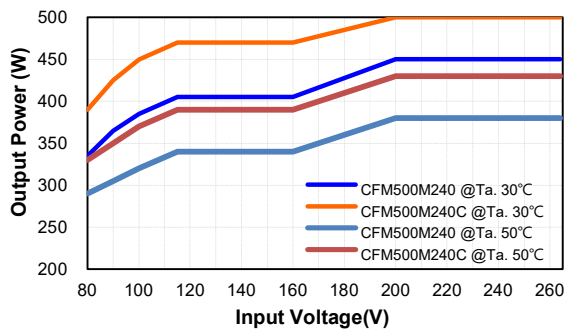
Output power & Input Voltage
