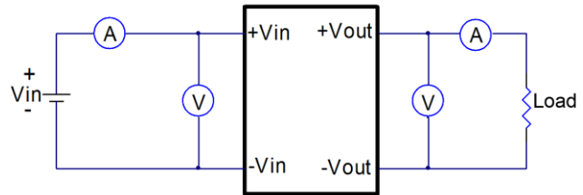
DH30W10 Series Test Setup
