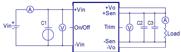
CQB75-300S Series Test Setup
