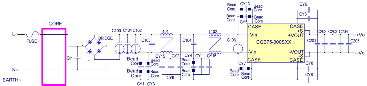
Figure1 Connection circuit
