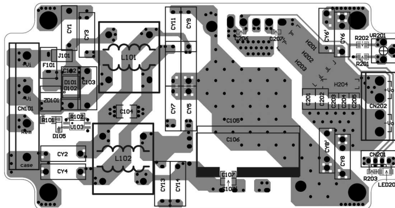
Figure2 PCB layout top view
