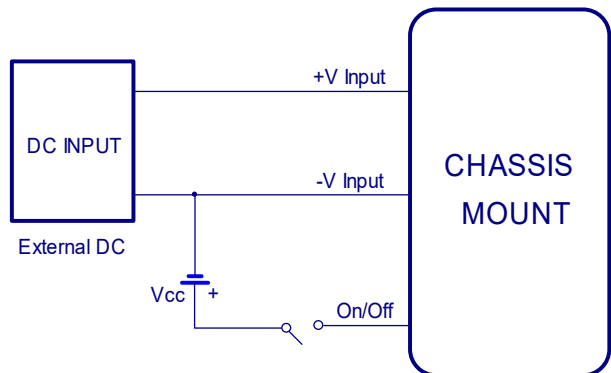
Remote On/Off Connection Example
