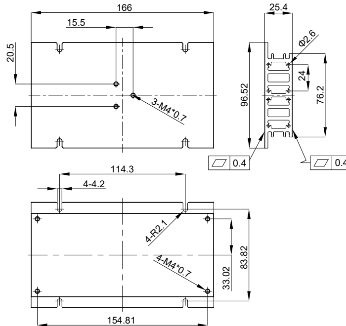
Heat Sink CMLH02
