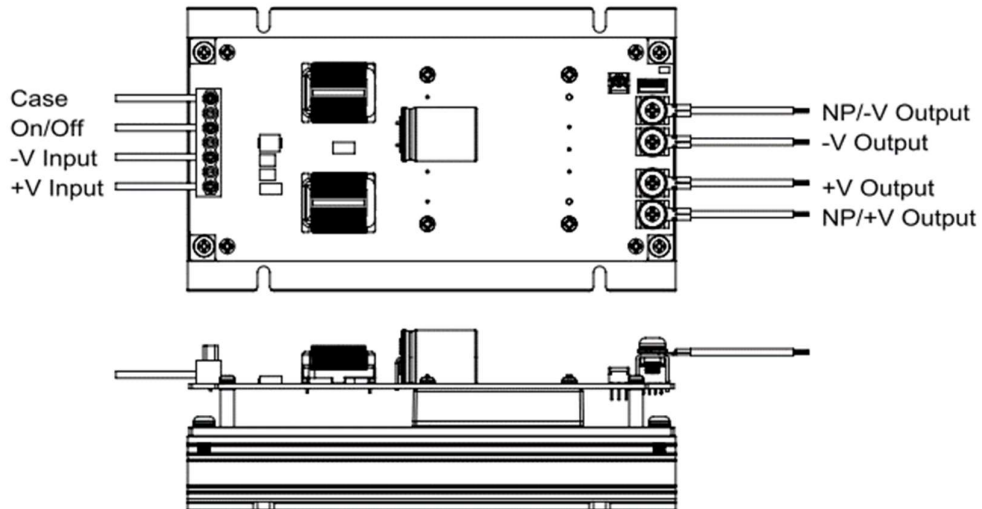
Figures 3 CHB300-300SXX-CMFC with Heat Sink CMLH02
