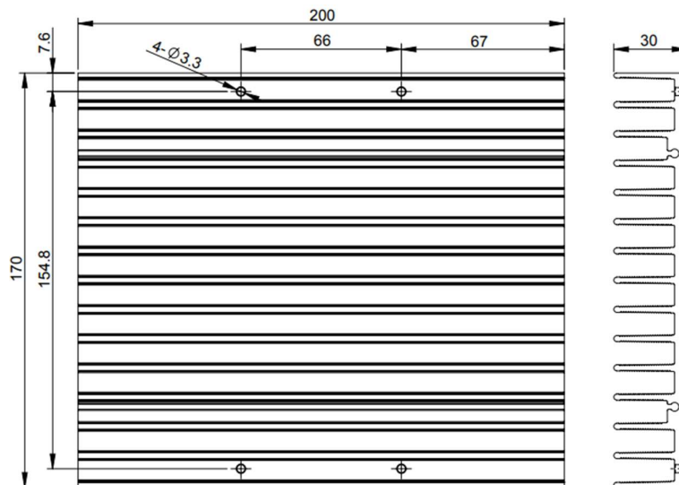
Heat Sink (7.87x6.7x1.18inch)
