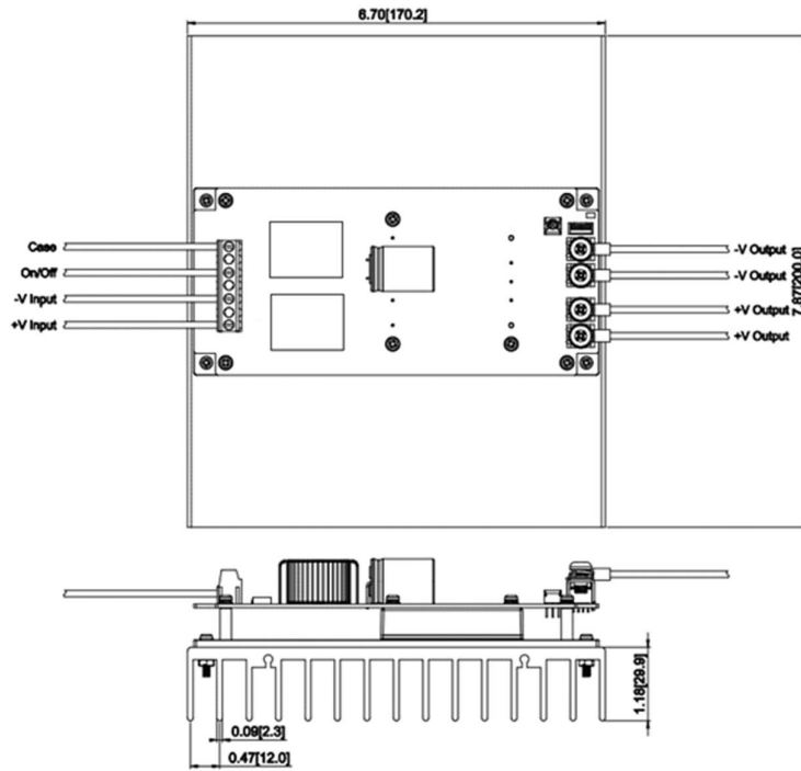
Figures 1 CHB300-300SXX-CMFC with Heat Sink (7.87x6.7x1.18inch)
