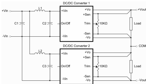
Simple \pm Output Operation Connect Circuit
